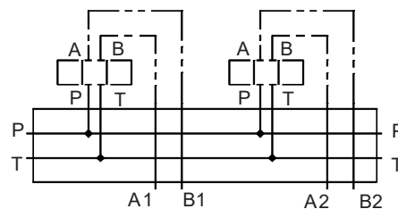
Hydraulic Circuit
